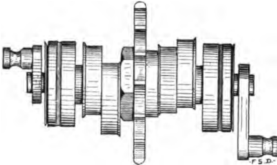
FIG. 245. —Crank Shaft of the "Locomobile" Steam Carriage, showing the cranks at both ends, the ball bearings and eccentrics, and the sprocket at the centre. Most steam carriage engines have similarly arranged crank shafts, although with several makes the entire mechanism is turned from one solid casting.
